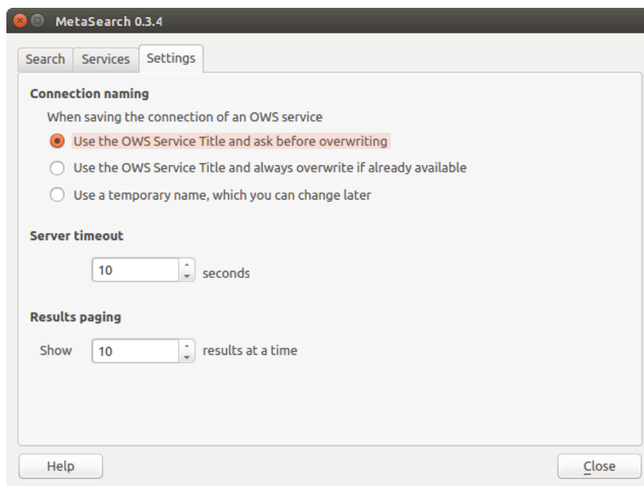
Figure 21.35: Metasearch setting
