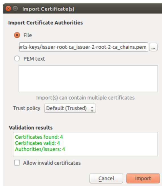
Figure 17.26: Import certificates dialog
