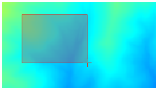
Figure 20.13: Extent Drag
