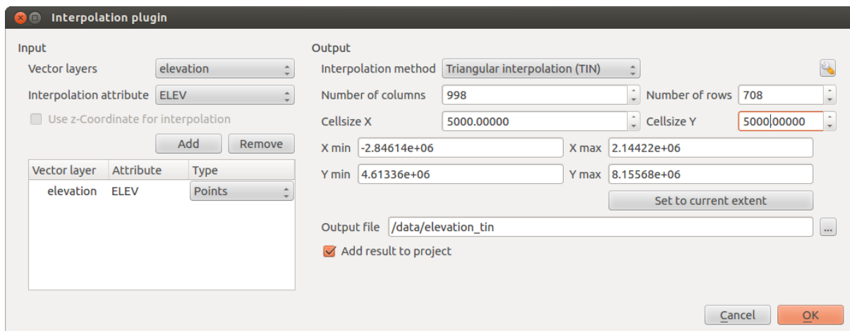
Figure 21.30: Interpolation Plugin
